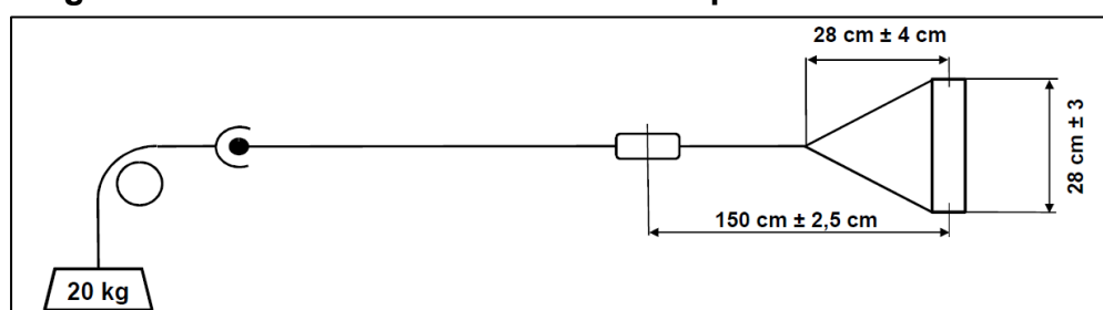
Diagram A1.5: Handle Dimensions in Jump and Slalom
