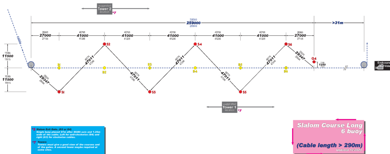
Diagram A3.2: S6 Slalom Course (long > 300m)
