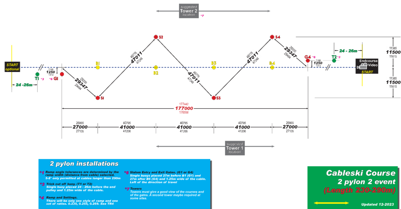
Diagram A6.1.2: 3-event short
