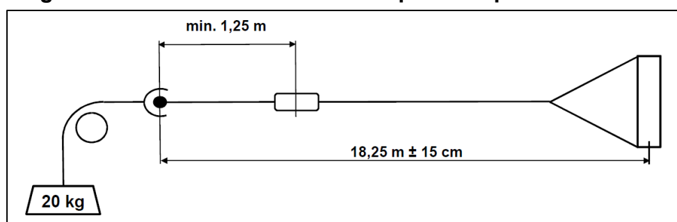
Diagram A1.6: Tow lines made with Spectra ropes
