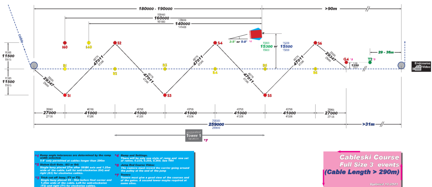
Diagram A6.3.1: Standard 3-event setup fullsize
